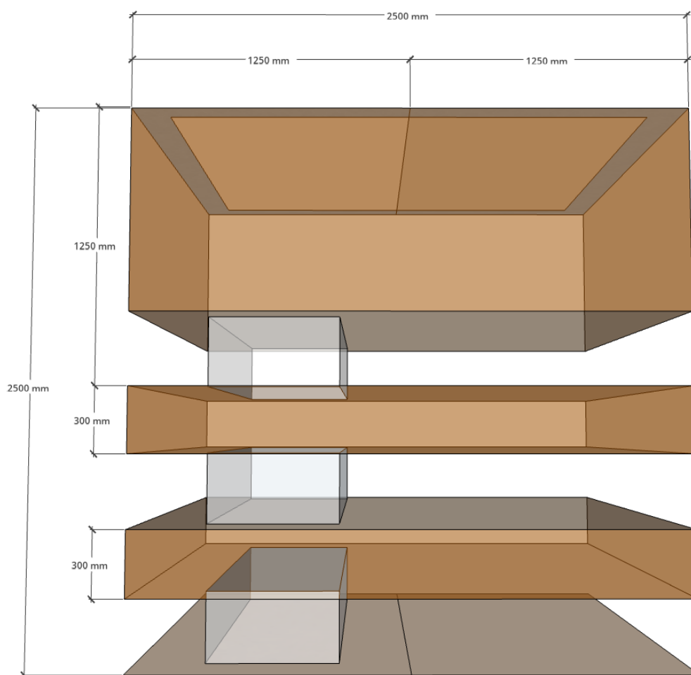
Fig. 1. Double plot of desirable 2.5m depth and 300mm separation distances required.
